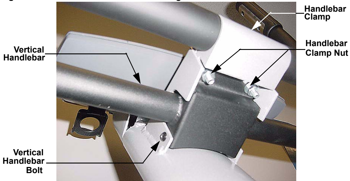
Diagram 7.8 - Vertical Handlebar Mounting
