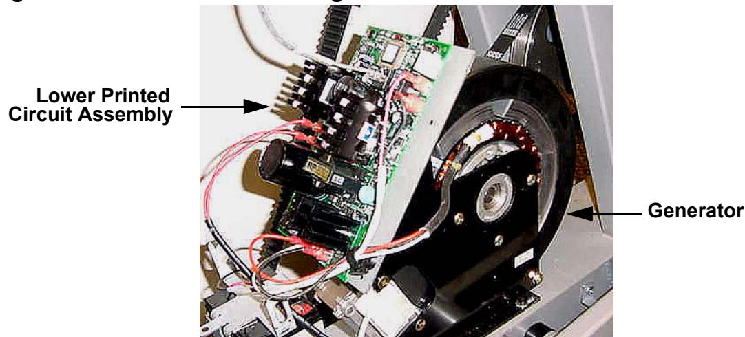
Diagram 7.13 - Generator Mounting
