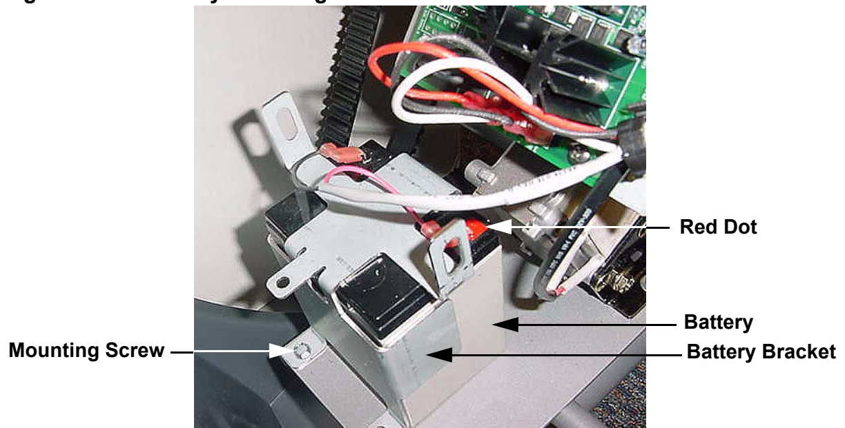
Diagram 7.16 - Battery Mounting
