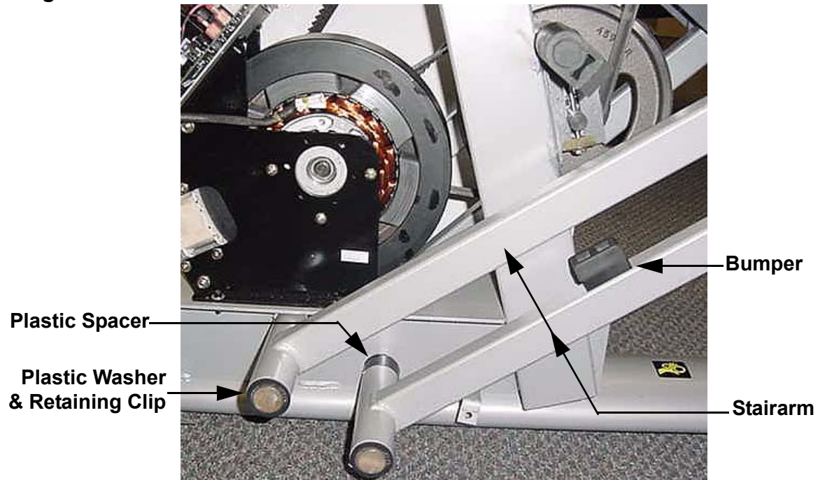
Diagram 7.12 - Stairarms
